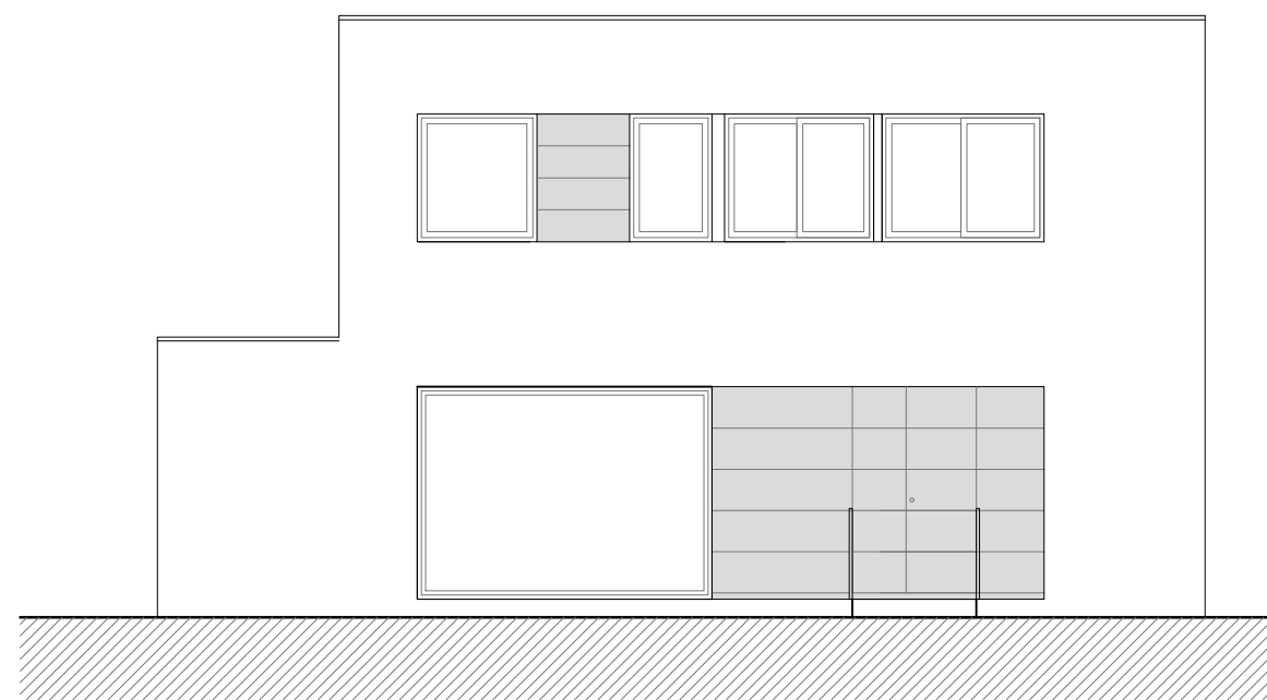
FAÇANA PRINCIPAL
