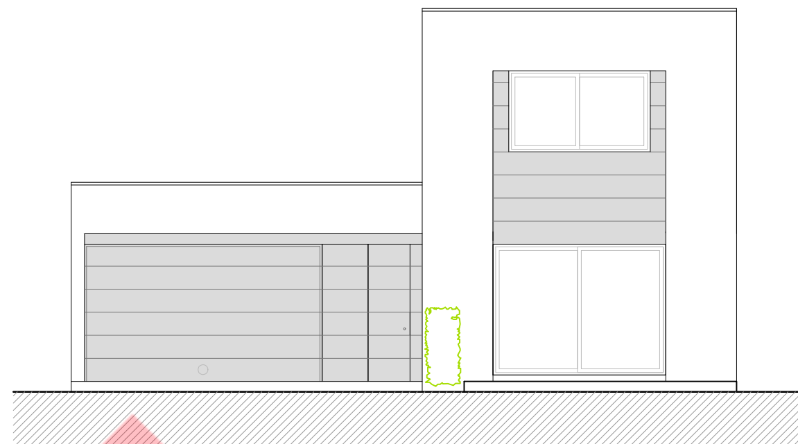
FAÇANA PRINCIPAL
